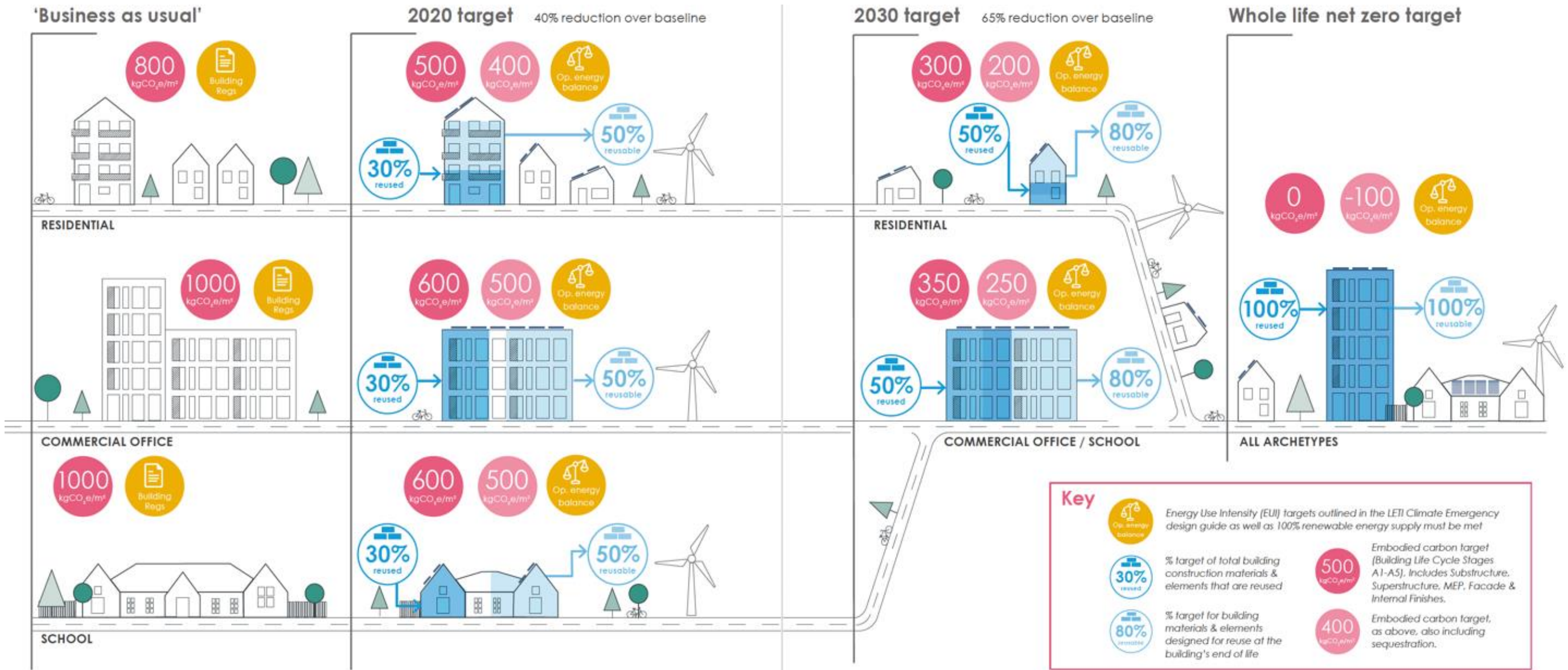
Figure 7.1 - LETI Embodied Carbon Reduction Targets towards Whole Life Net Zero
