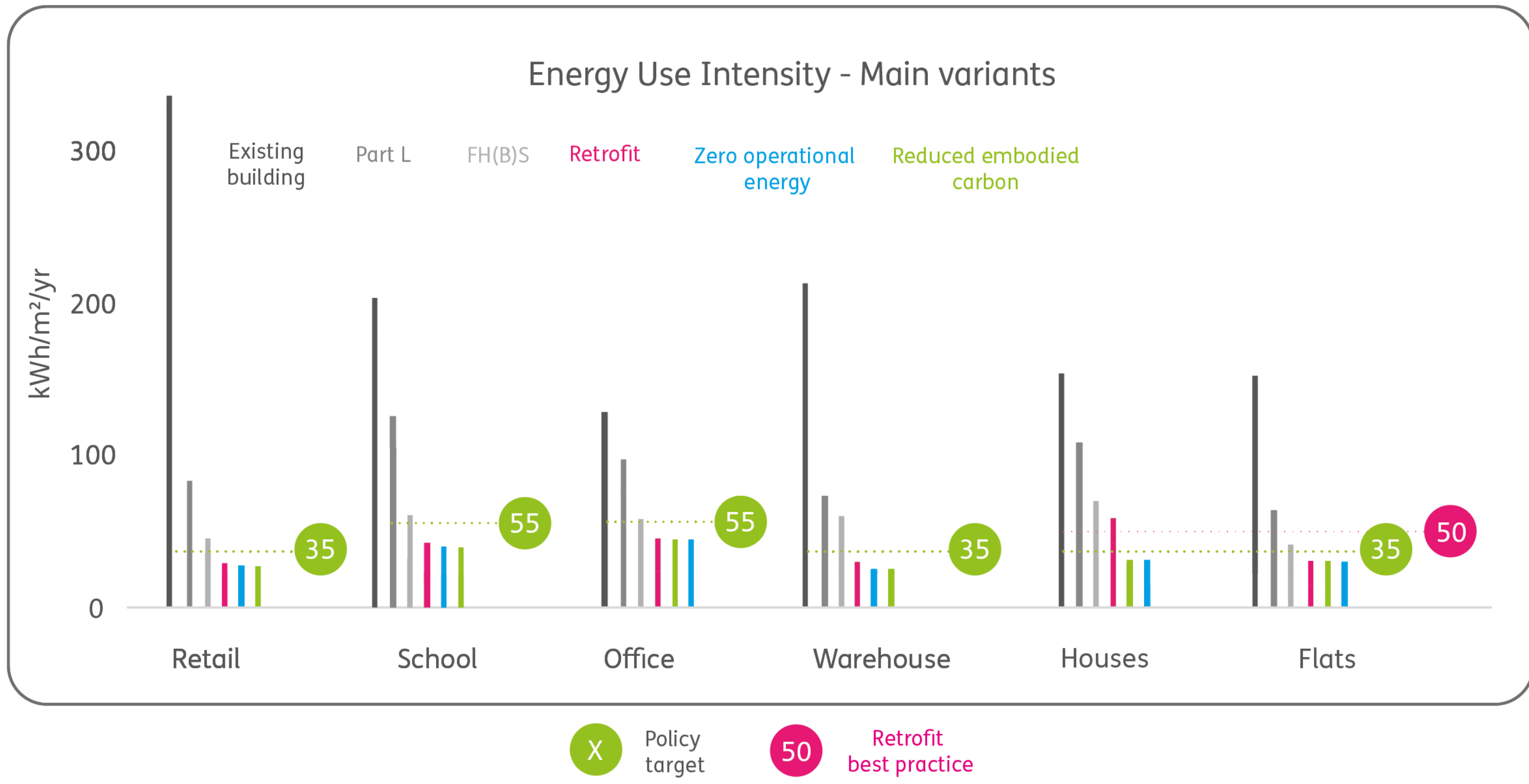
Figure 15. Energy use intensity graph for domestic and non-domestic archetypes
