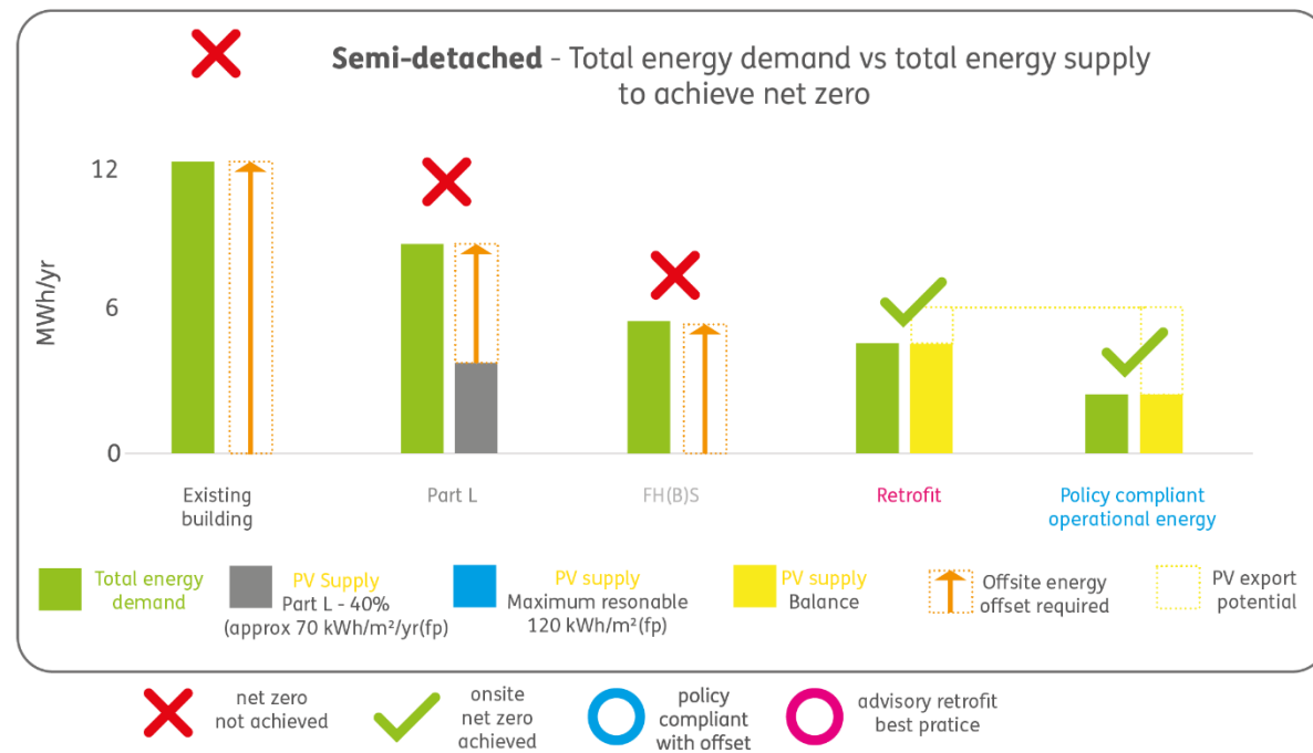
Figure 18. Graph showing the energy balance of the semi-detached archetype variants
